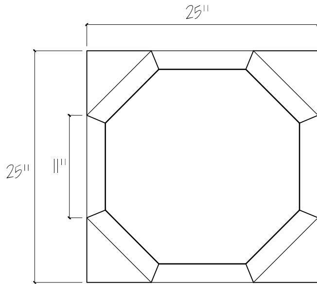
Plan/ Top View
